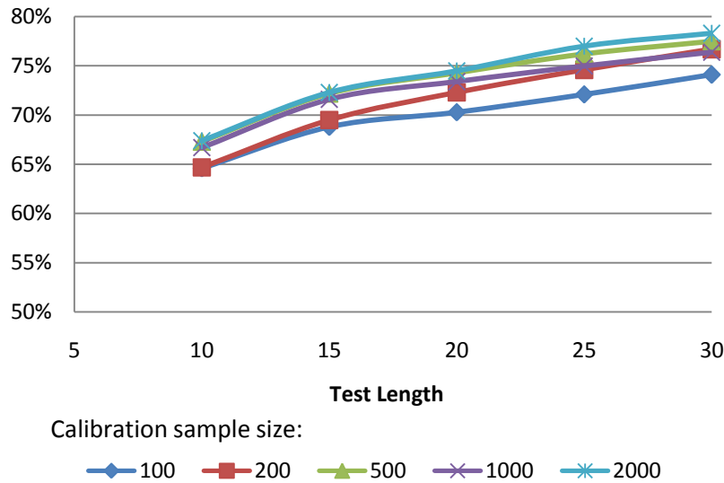
Classification accuracy as a function of test length and calibration sample size
